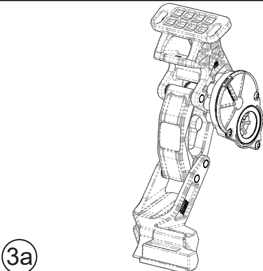
Driver Motor Linkage assembly
